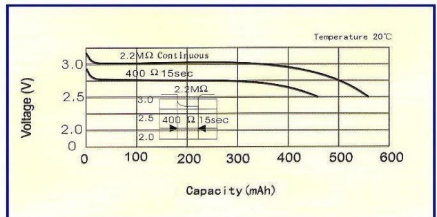
Pulse Discharge Characteristics
