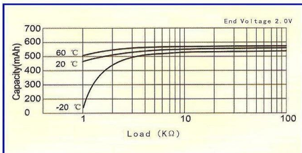
Load-capacity
